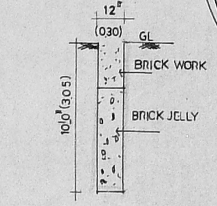
PERCOLATION PIT DETAILS
